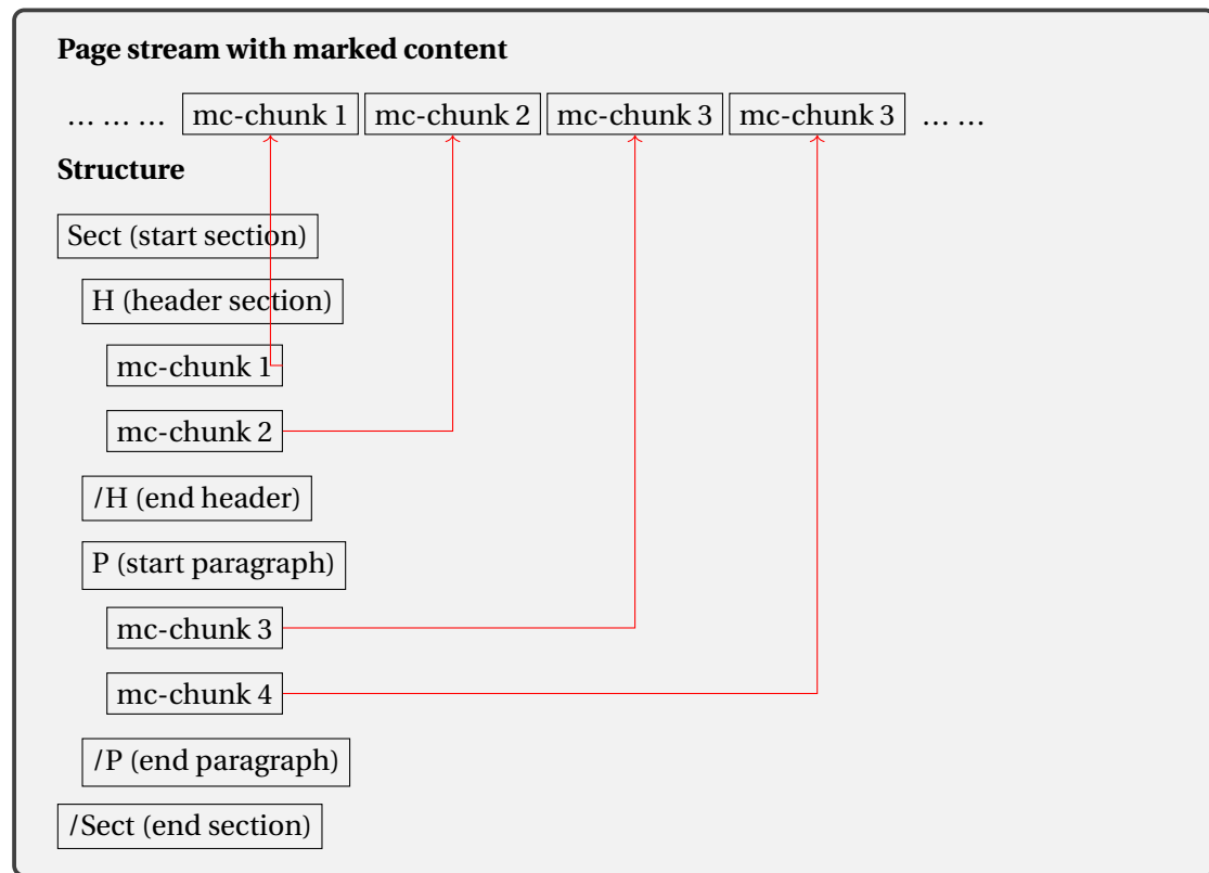
Figure 4: Schematical description of the relation between marked content in the page stream and the structure
